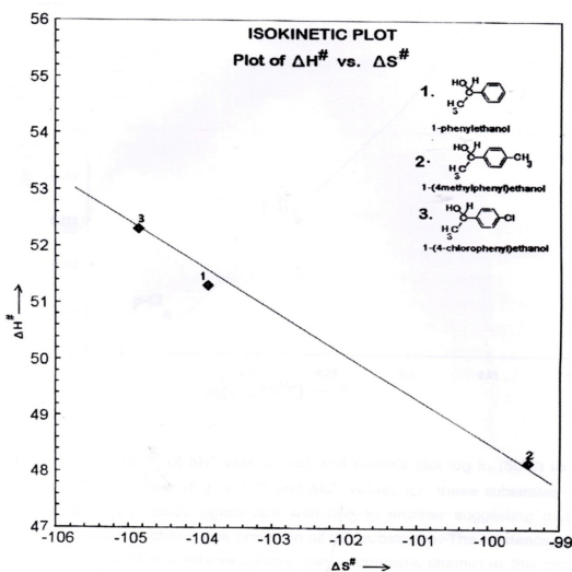
Figure-1. Benzyl alcohols oxidations are linearly related by plotting " \Delta H^\ddagger vs. " \Delta S^\ddagger "
