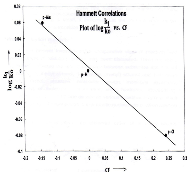
Figure 3. Hammett Correlation plot given substituent.
