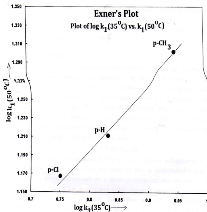
Figure 2. The iso-kinetic plot of " H^\ddagger versus - " S^\ddagger " and Exner's plot \log k_1(50^\circ\text{C}) vs. \log k_1(35^\circ\text{C}) , are linear (Figure 2) and " G^\ddagger " values for these substrates – \text{SeO}_2 system.
