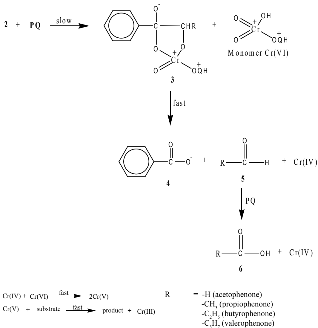
Scheme 2 Mechanistic pathway of formation of the Cr(IV) species.
