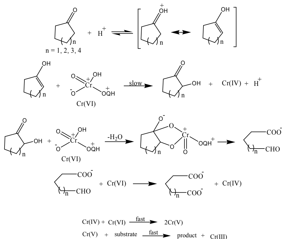
Scheme 1 Rate determining step of the oxidant on the enol form of the substrate.
